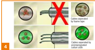
4 Apply a suitable barrier material foam tape or cotton cloth. When several cables are fed through, they must be separated from each other by the barrier material for better application
